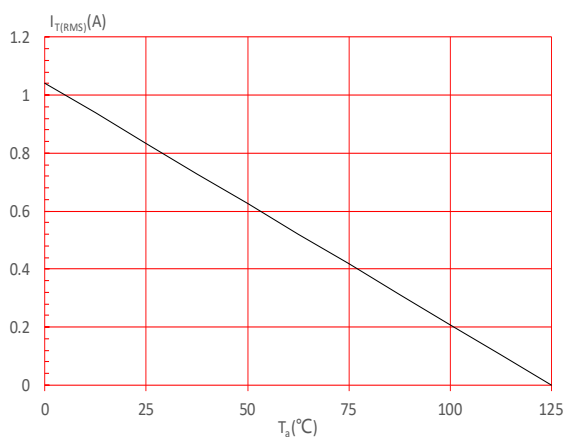
FIG.5: On-state characteristics
