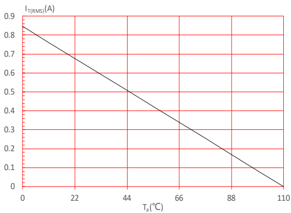
FIG.5: On-state characteristics
