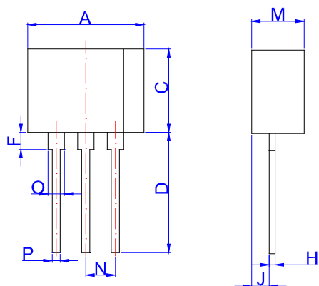
TO-202-3
