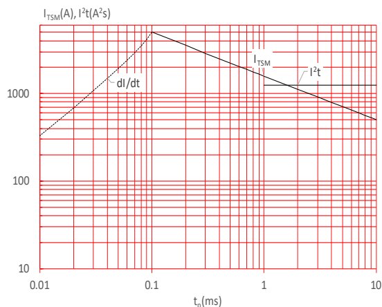
FIG.6: Non-repetitive surge peak on-state current for a sinusoidal pulse with width t_p < 10ms , and corresponding value of I^2t ( dI/dt < 150A/\mu s )
