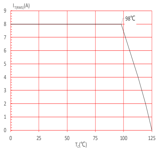
FIG.4: On-state characteristics
