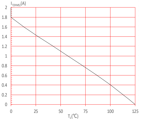
FIG.4: On-state characteristics
