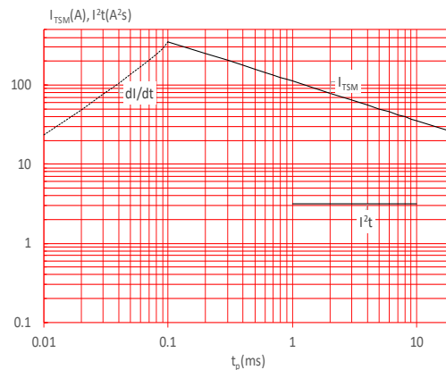
FIG.6: Non-repetitive surge peak on-state current for a sinusoidal pulse with width t_p < 20ms , and corresponding value of I^2t ( di/dt < 100A/μs )
