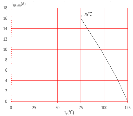
FIG.4: On-state characteristics
