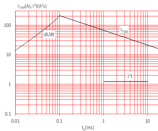
FIG.6: Non-repetitive surge peak on-state current for a sinusoidal pulse with width t_p < 20\text{ms} , and corresponding value of I^2t ( di/dt < 60\text{A}/\mu\text{s} )
