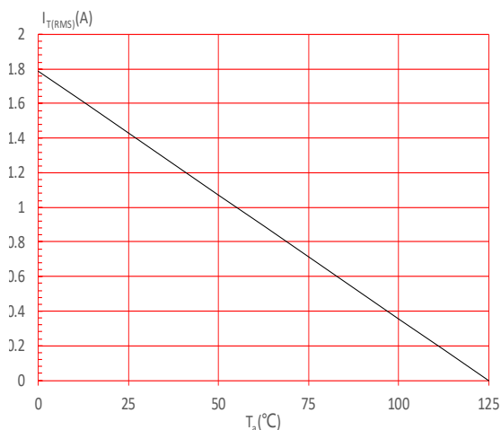
FIG.5: On-state characteristics
