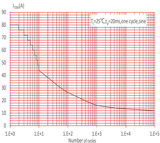
FIG.6: Non-repetitive surge peak on-state current for a sinusoidal pulse with width t_p < 20ms , and corresponding value of I^2t ( dl/dt < 100A/μs )
